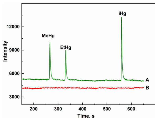
Figure 2. Typical chromatograms of PCs HS-SPME-GC-DBD-OES for a mercury standard solution containing 15 \mu\text{g L}^{-1} iHg, MeHg, and EtHg (a) and a blank solution (b).
