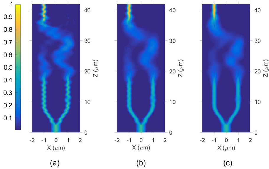
Fig. 7. Field distribution of the designed ultra-broadband DE/MUX when \text{TE}_0 mode is injected through the multimode waveguide (port 3) at wavelengths 1.4 \mu\text{m} (a), 1.55 \mu\text{m} (b) and 1.7 \mu\text{m} (c).
