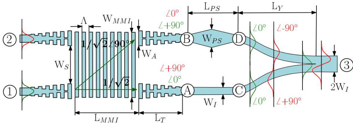
Fig. 2. Schematic and principle of operation of the proposed two-mode converter and DE/MUX based on a SWG-MMI, a symmetric Y-junction and a 90° phase shifter.
