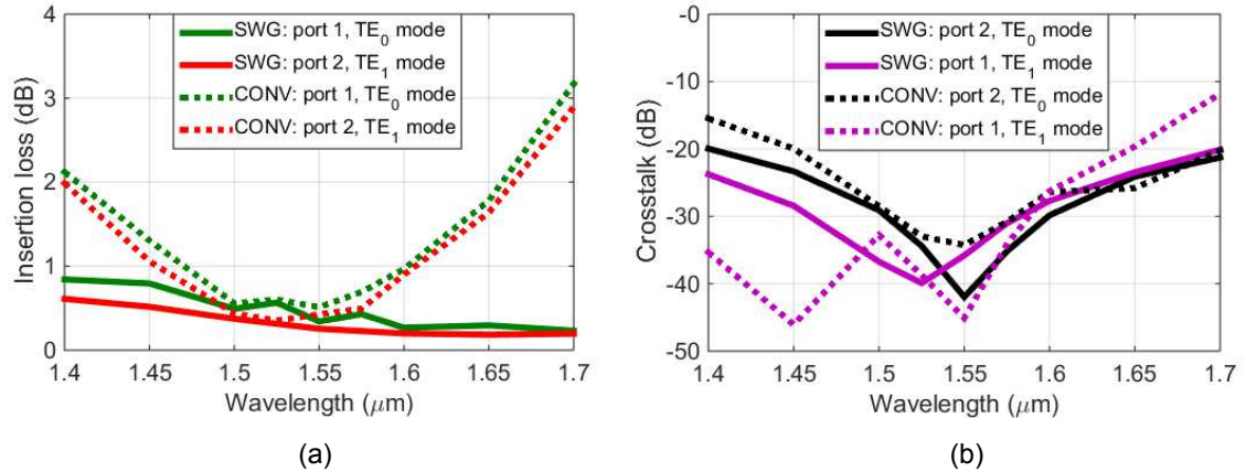
Fig. 6. Comparison of the insertion losses (a) and crosstalk (b) of our proposed device (solid curves) and the conventional equivalent device (dotted curves). Worst case has been taken into account, i.e. maximum of insertion losses and crosstalk for MUX and DEMUX configurations.
