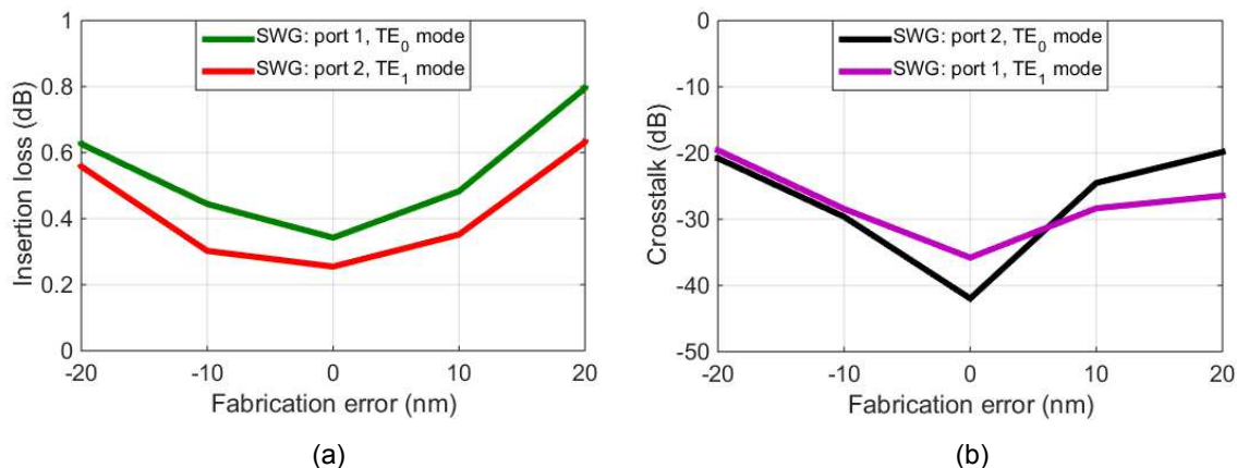
Fig. 9. Insertion losses (a) and crosstalk (b) for the worst case of the proposed ultra-broadband two-mode converter and DE/MUX as a function of fabrication error at \lambda = 1.55 \mu\text{m} . Worst case has been taken into account, i.e. maximum of insertion losses and crosstalk for MUX and DEMUX configurations.
