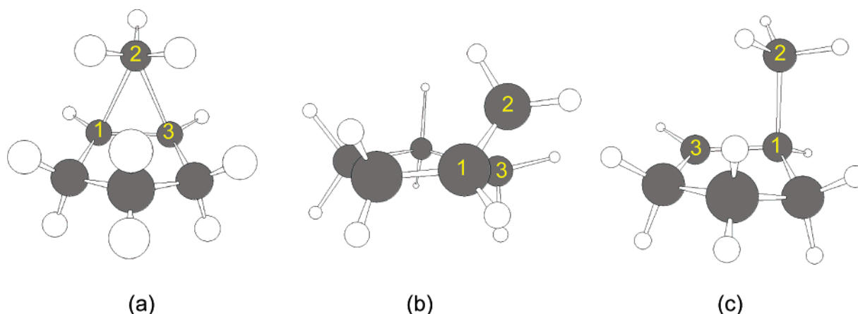
Figure 4. Selected structures erroneously predicted by other theoretical approaches. (a) I_{\text{int}} (MP2), (b) TS I p →I d (MP2), (c) I_{\text{int}} (MP2).
