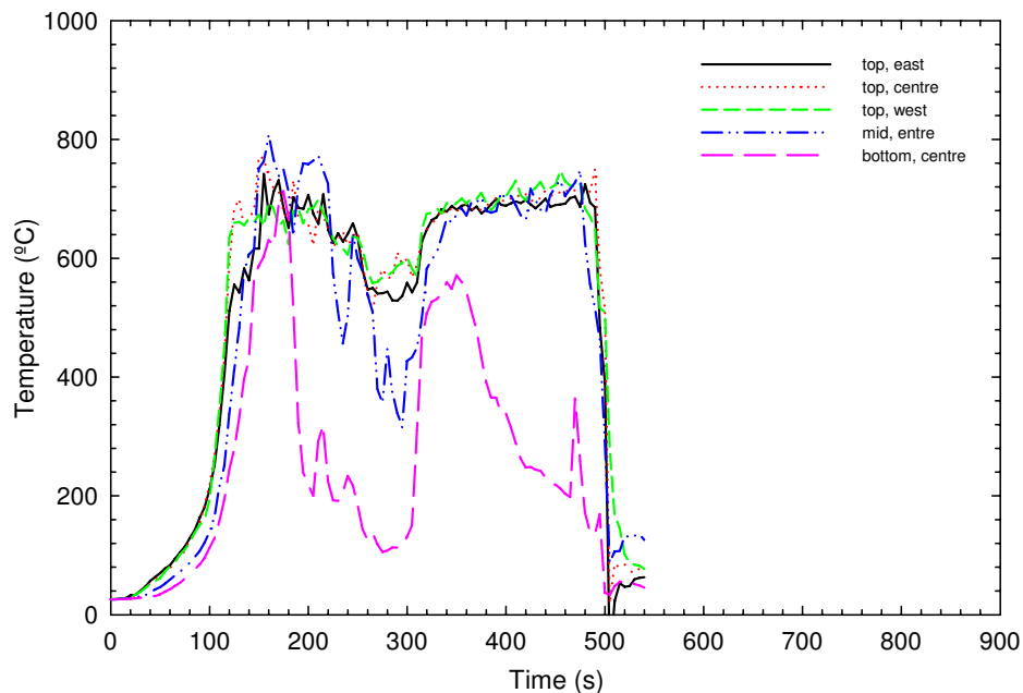
Figure 23. Temperatures at the window in the basement for UF-05
