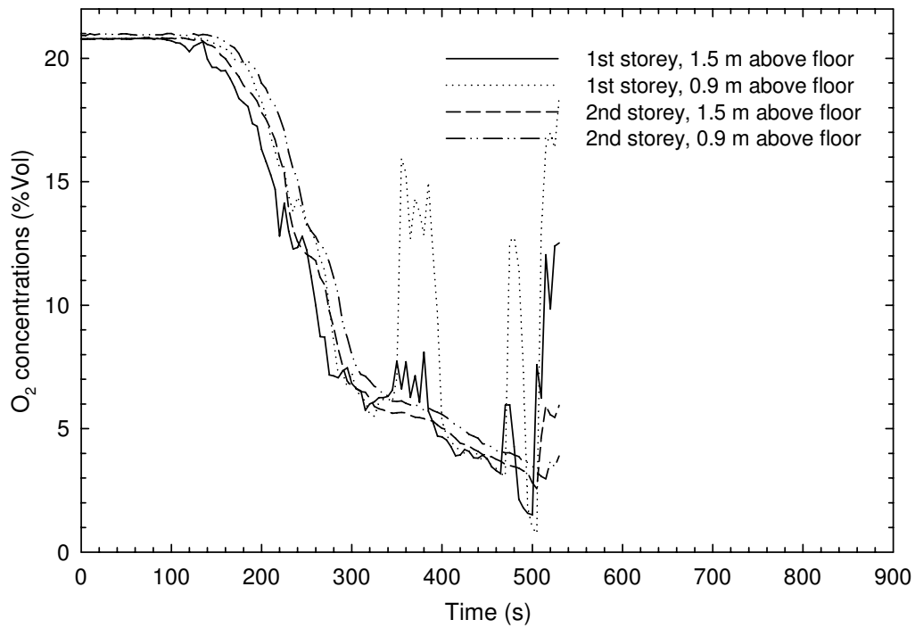
Figure 33. O 2 measurements for Test UF-05
