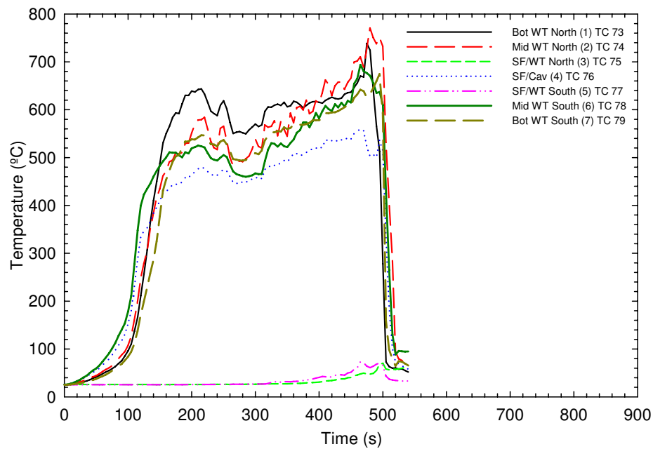
j) Thermocouples in cavity C-13
