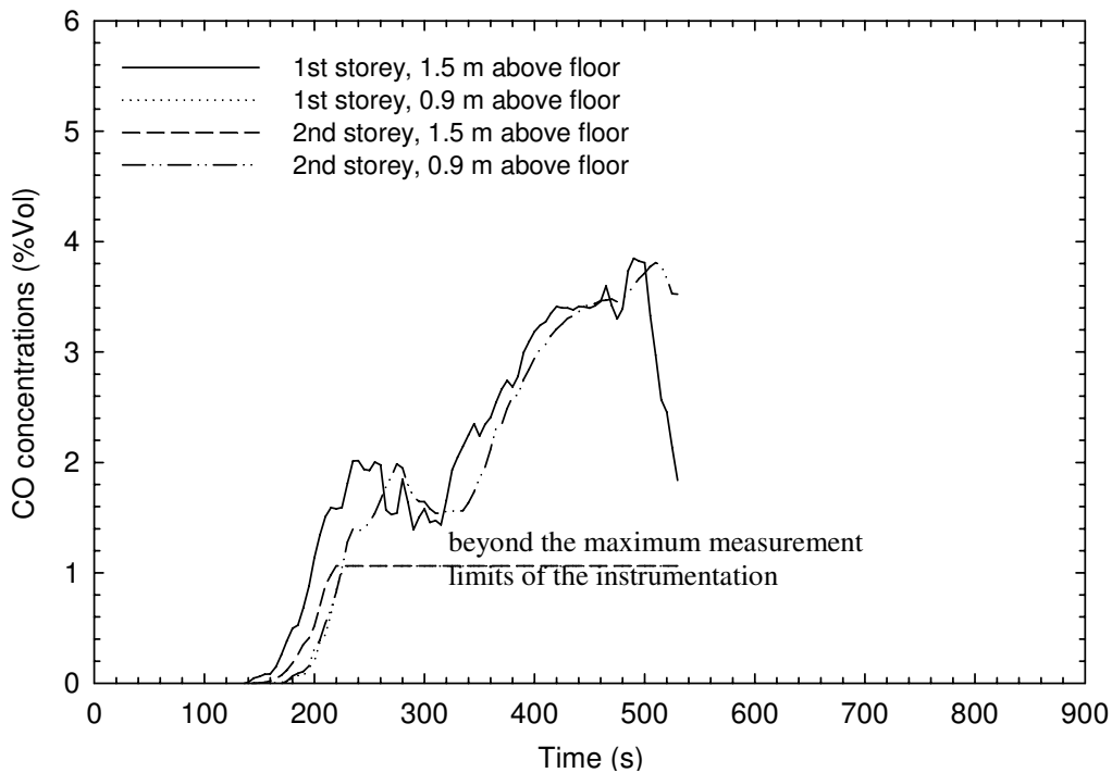
Figure 32. CO measurements for Test UF-05
