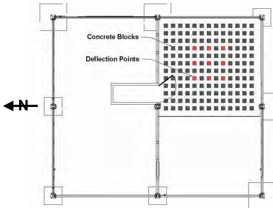
Figure 18. Loading blocks and locations of the deflection measurement points on the unexposed side of the floor
