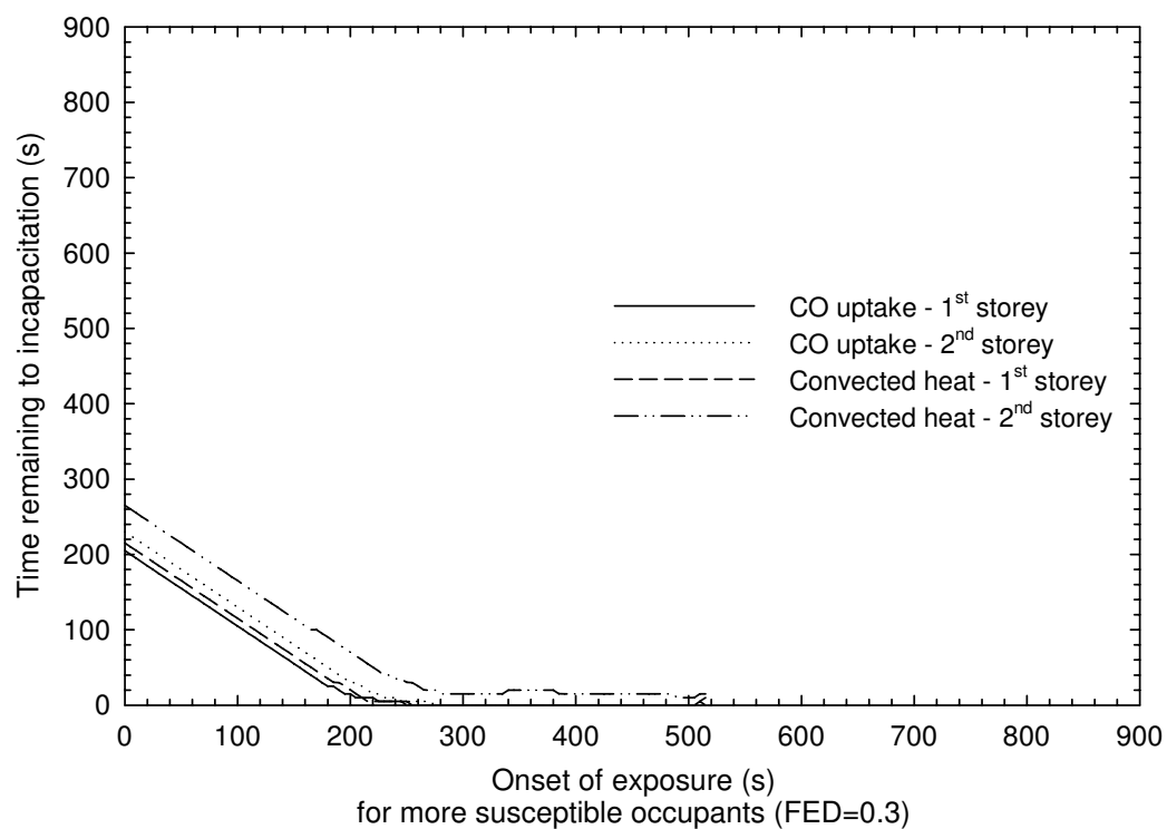
Figure 36. Time remaining to incapacitation versus onset of exposure for Test UF-05 (ignition at time zero)
