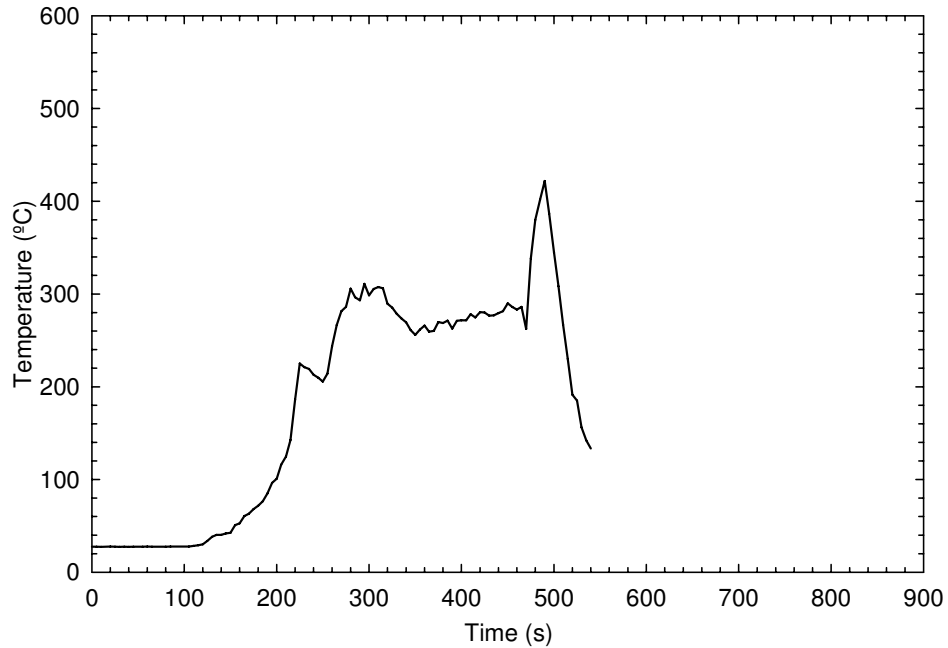
Figure 26. Temperatures at the outside doorway on the first storey for UF-05
