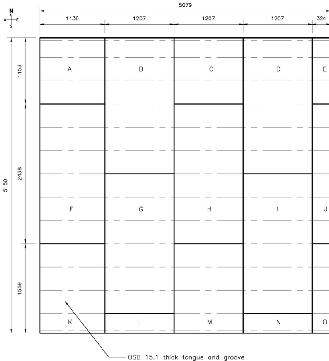
Figure 13. Subfloor layout details (all dimensions in mm)
