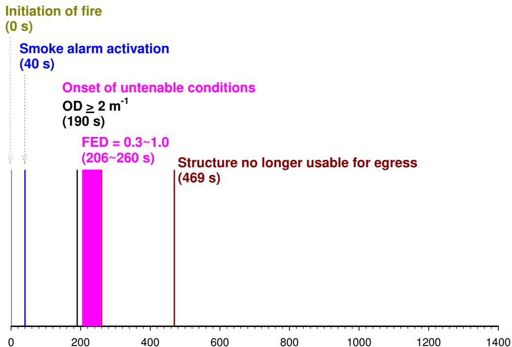
Figure 37. Sequence of fire events in Test UF-05 (s)
