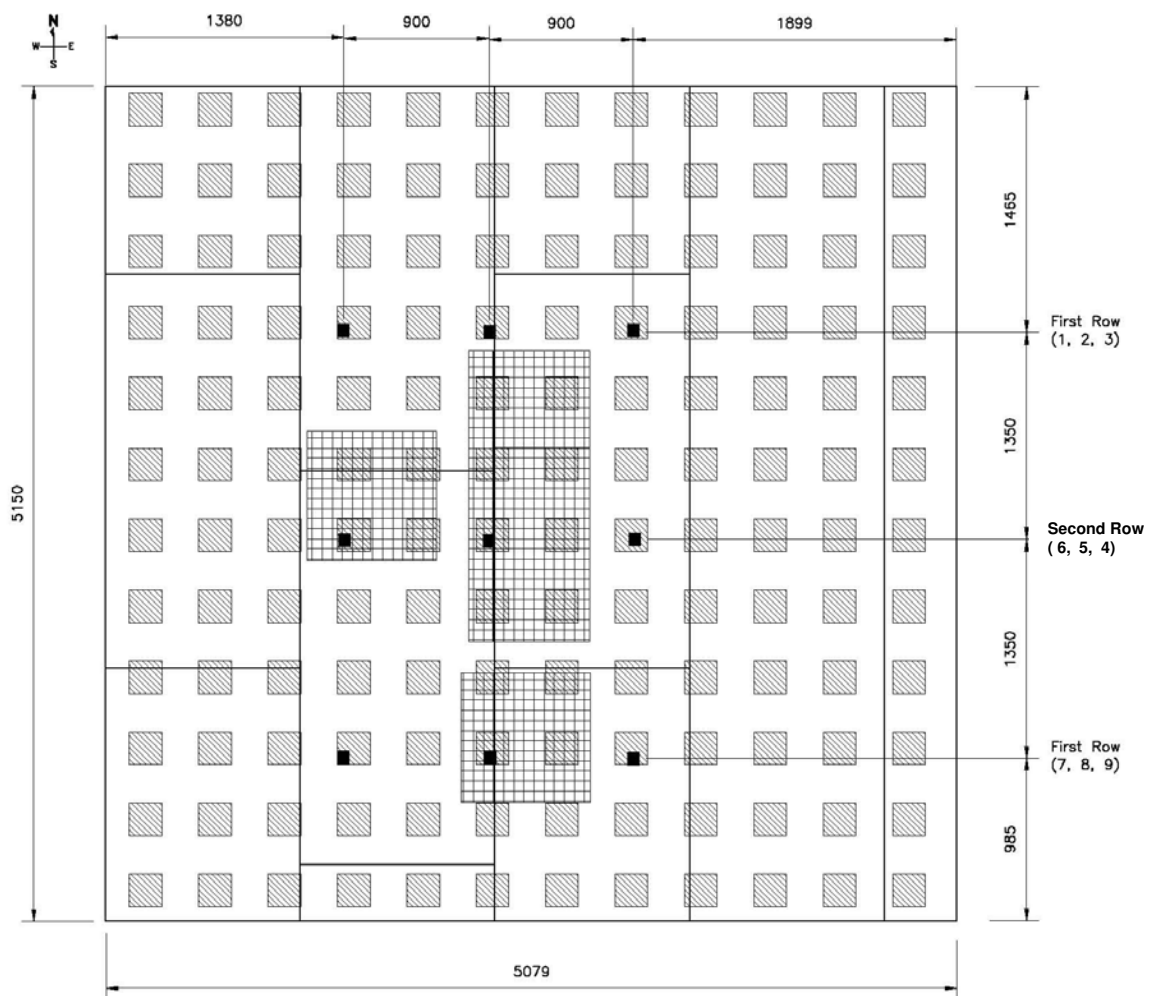
Figure 29. Deflection points measured (all dimensions in mm)
