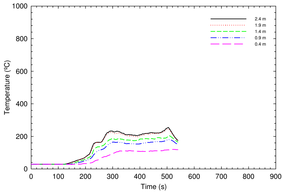
Figure 25. Temperatures on the second storey at the stairs for UF-05
