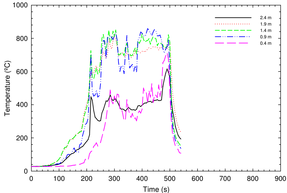
Figure 24. Temperatures on the first storey at the top of the stairs from the basement for UF-05
