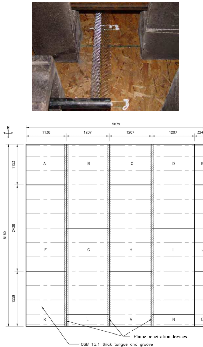
Figure 17. Wire mesh device to detect flame penetration
