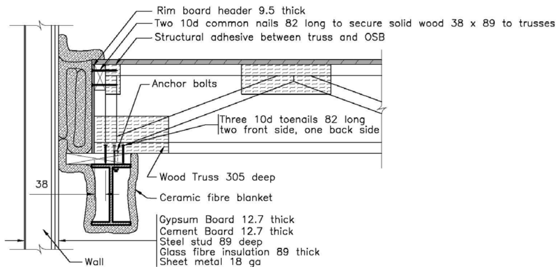
Figure 12. End connection details and supports (all dimensions in mm)
