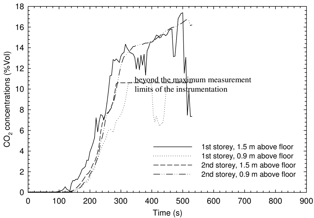
Figure 34. CO 2 measurements for Test UF-05
