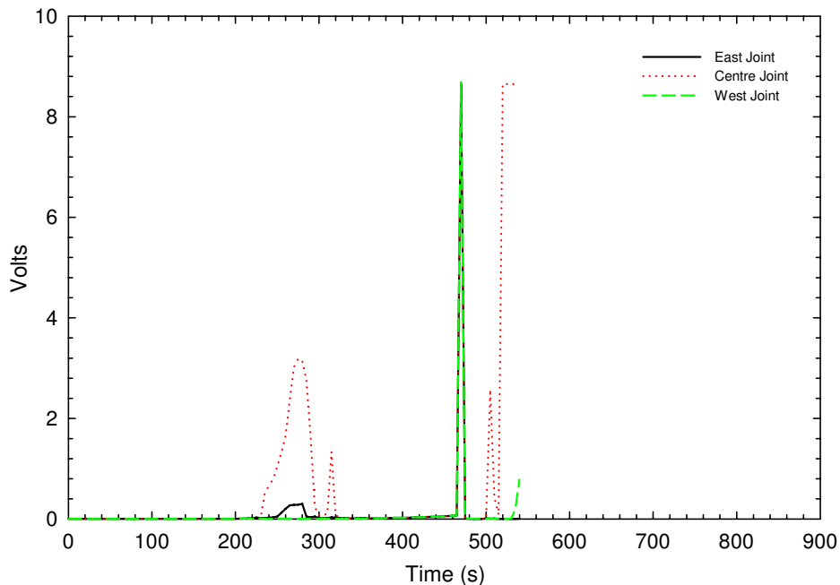
Figure 31. Results of flame sensors at different joints
