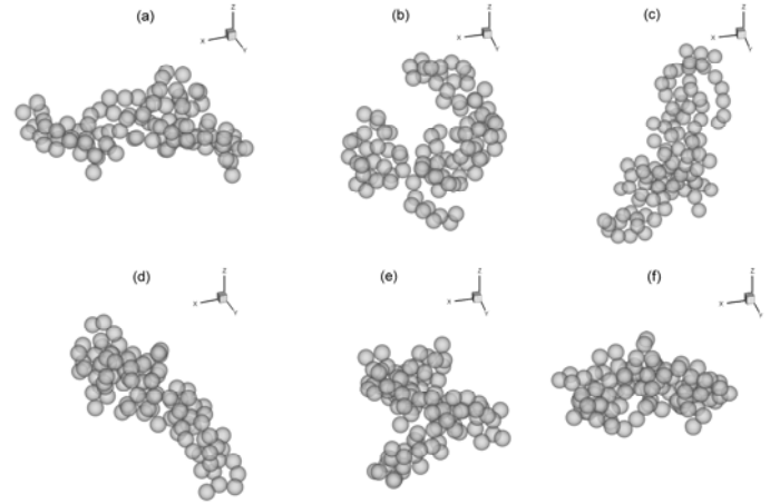
Fig. 1 The first six realizations for N = 100 .
