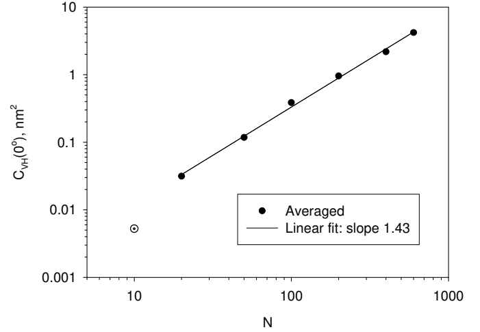
Fig. 6 Variation of configuration- and orientation-averaged C_{VH}(0^\circ) with aggregate size N .
