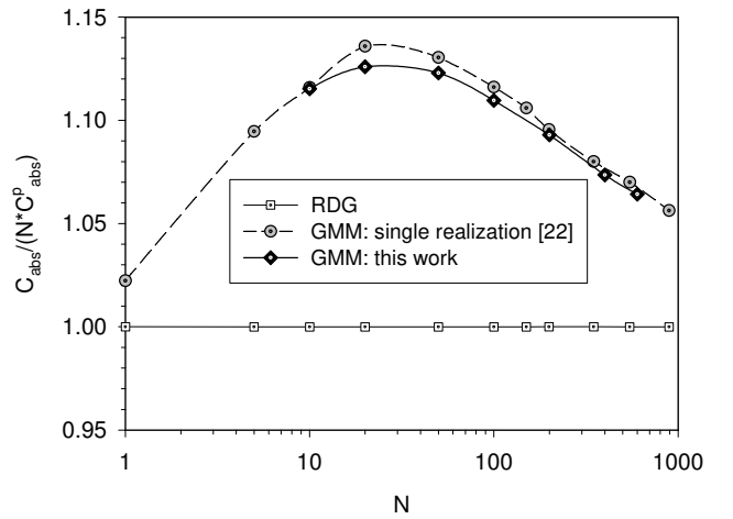
Fig. 2 Comparison of nondimensional aggregate absorption cross section.
