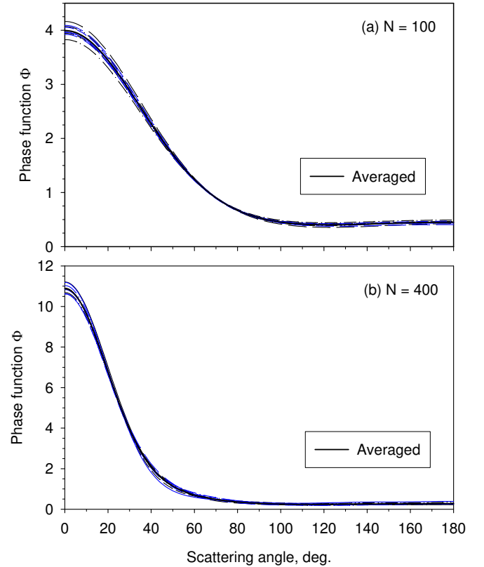
Fig. 5 Scattering phase functions for different aggregate realizations and N = 100 and 400 .
