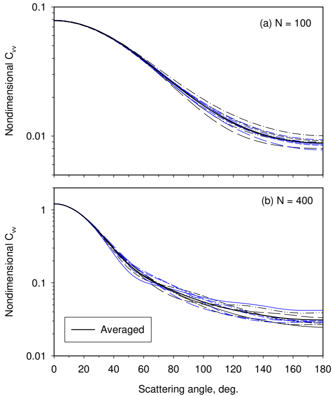
Fig. 4 Nondimensional vertical-vertical differential scattering cross sections for different aggregate realizations and N = 100 and 400 .
