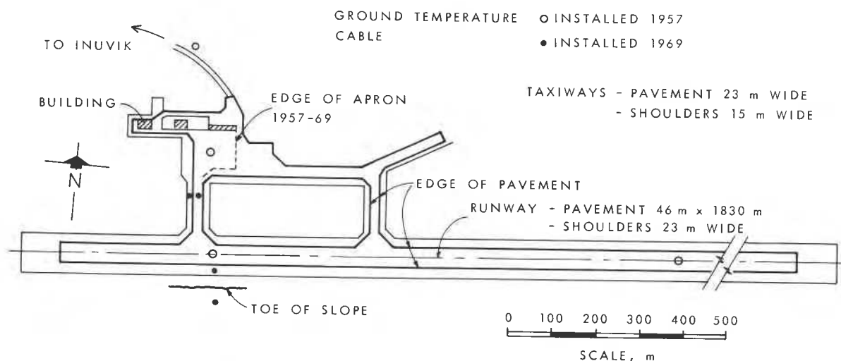
FIGURE 1. Plan showing general layout of the Inuvik, N.W.T., airstrip.
