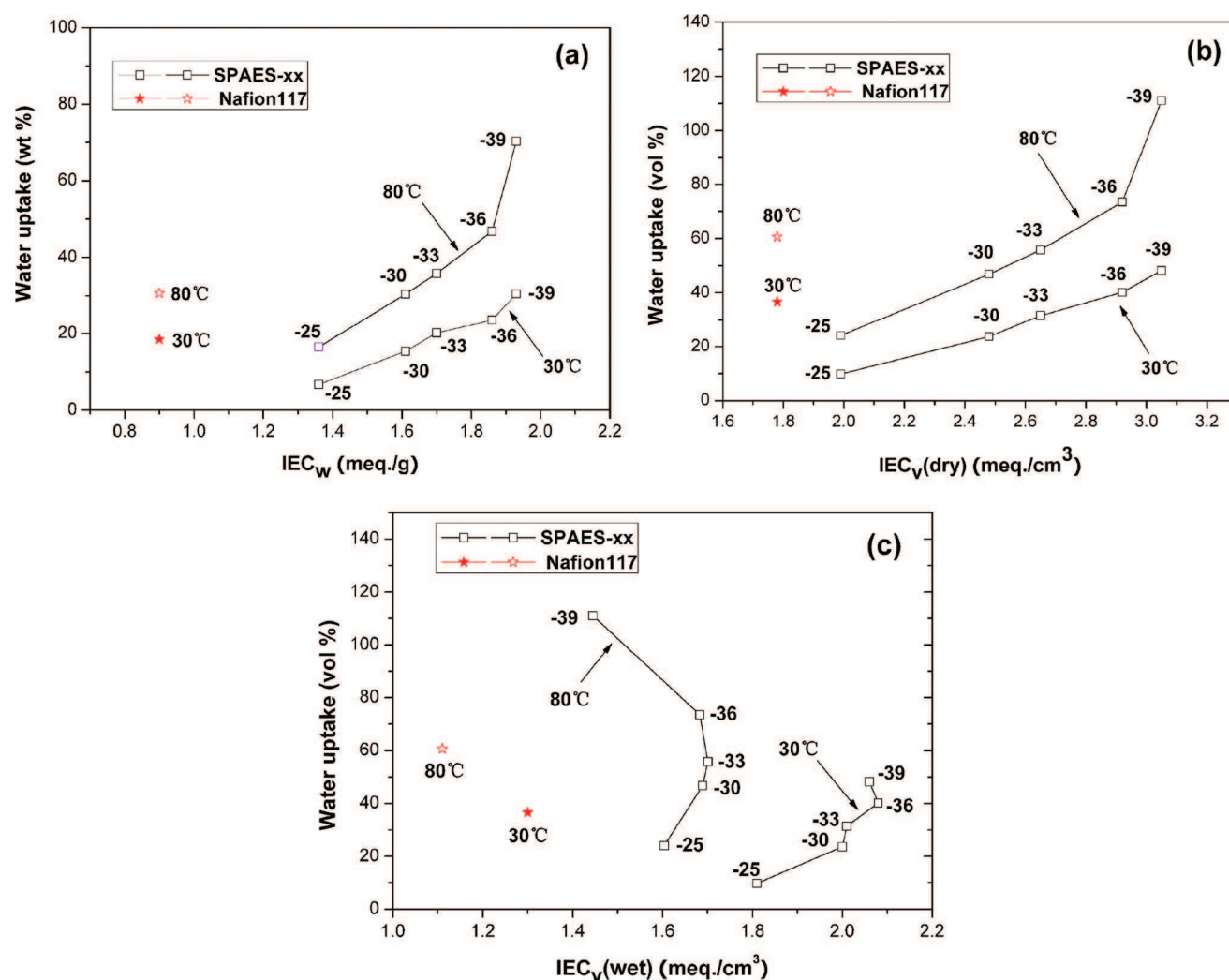
Figure 5. Water uptake dependence of IEC ( \text{IEC}_w ), \text{IEC}_v (dry), and \text{IEC}_v (wet) values of SPAES-xx membranes.
