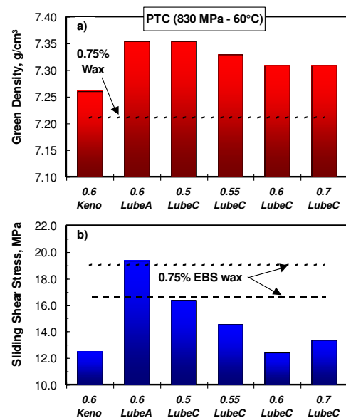
Figure 3. Compressibility (a) and ejection (b) of FN0205 mixes with various levels of lube C in the PTC.
