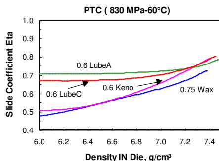
Figure 2. Slide coefficient as a function of density in the Die (FN0205 mixes).
