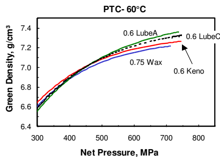
Figure 1. True Compressibility curves for FN0205 mixes.
