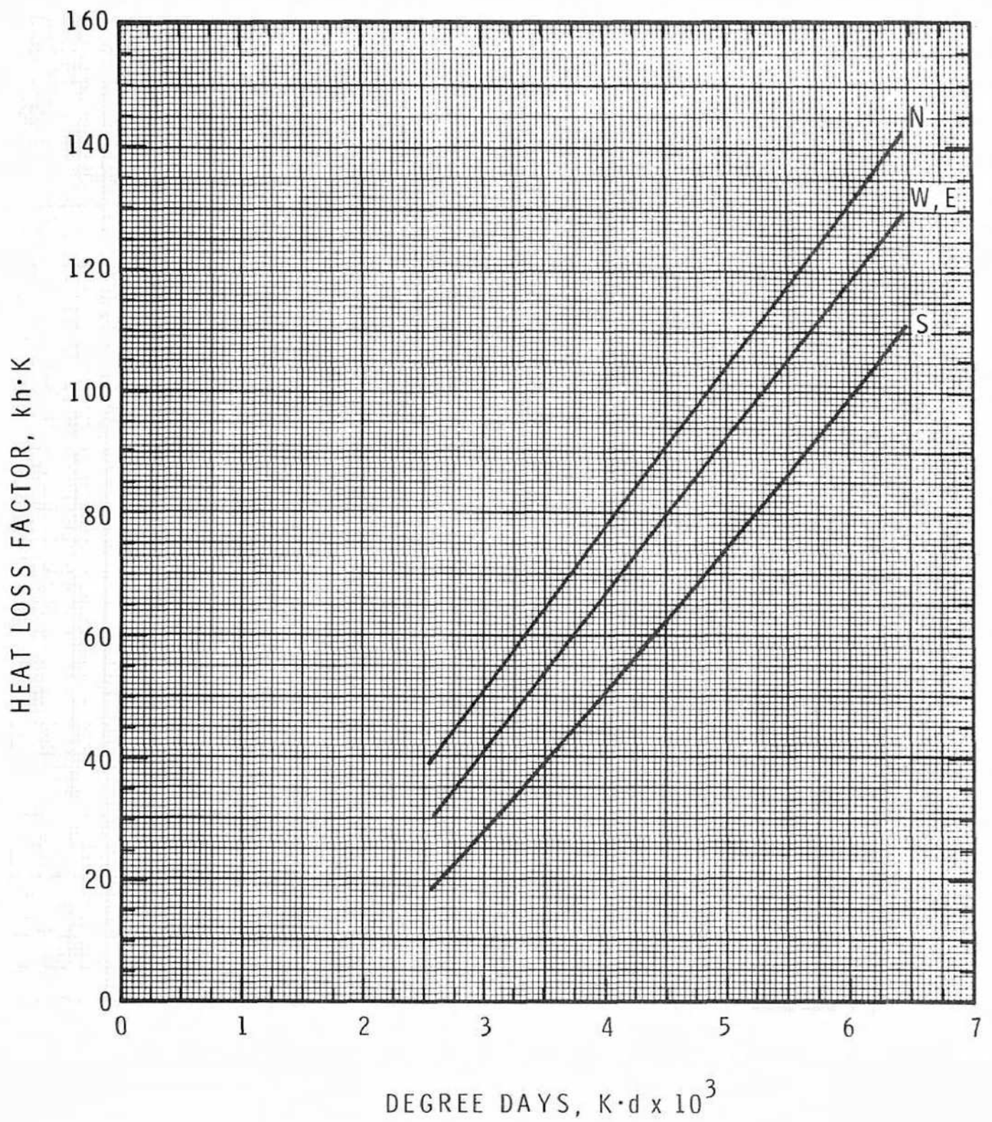
FIGURE 5 WALL HEAT LOSS FACTORS (EXTERIOR SURFACE COLOUR - MEDIUM)
