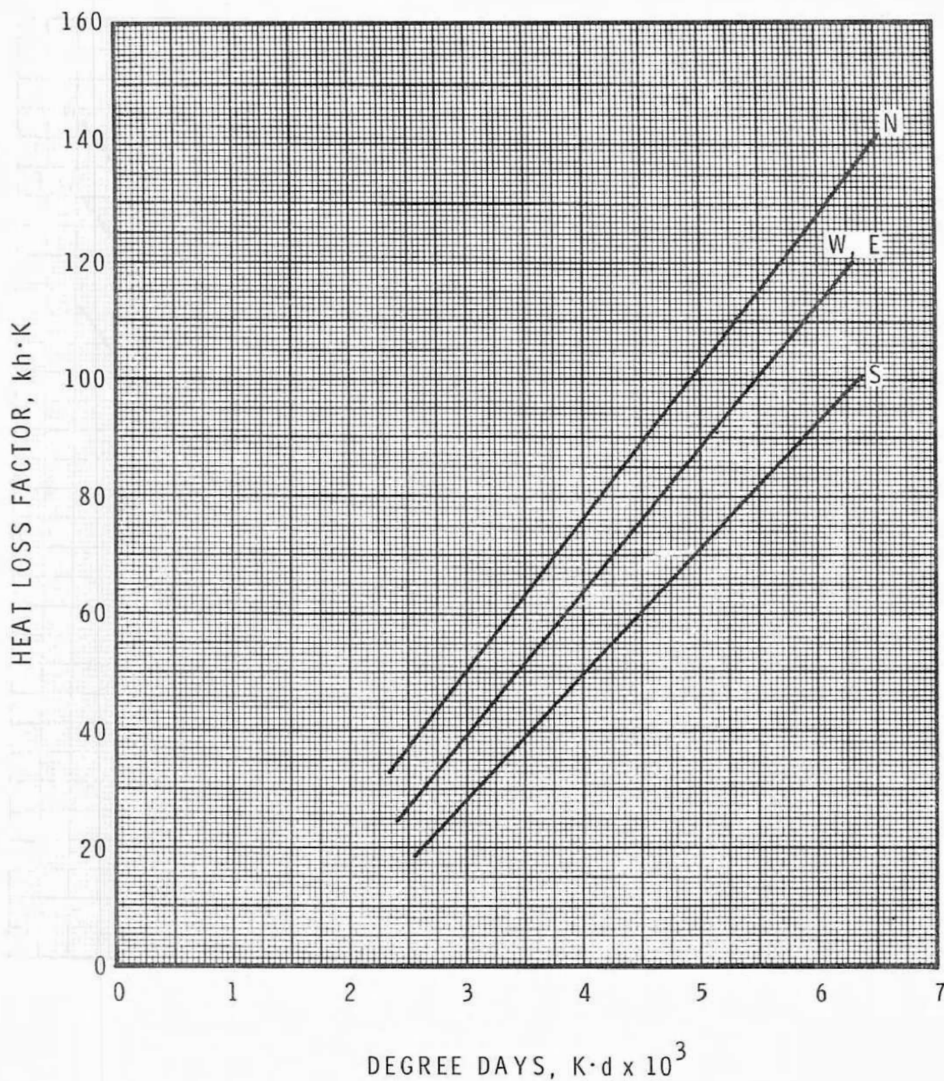
FIGURE 6 WALL HEAT LOSS FACTORS (EXTERIOR SURFACE COLOUR - DARK)
