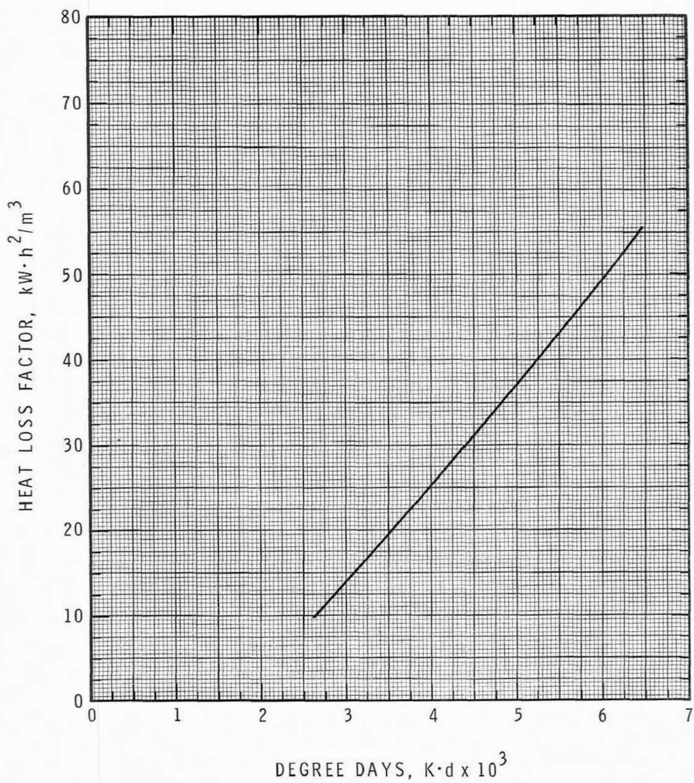
FIGURE 8 INFILTRATION HEAT LOSS FACTOR
