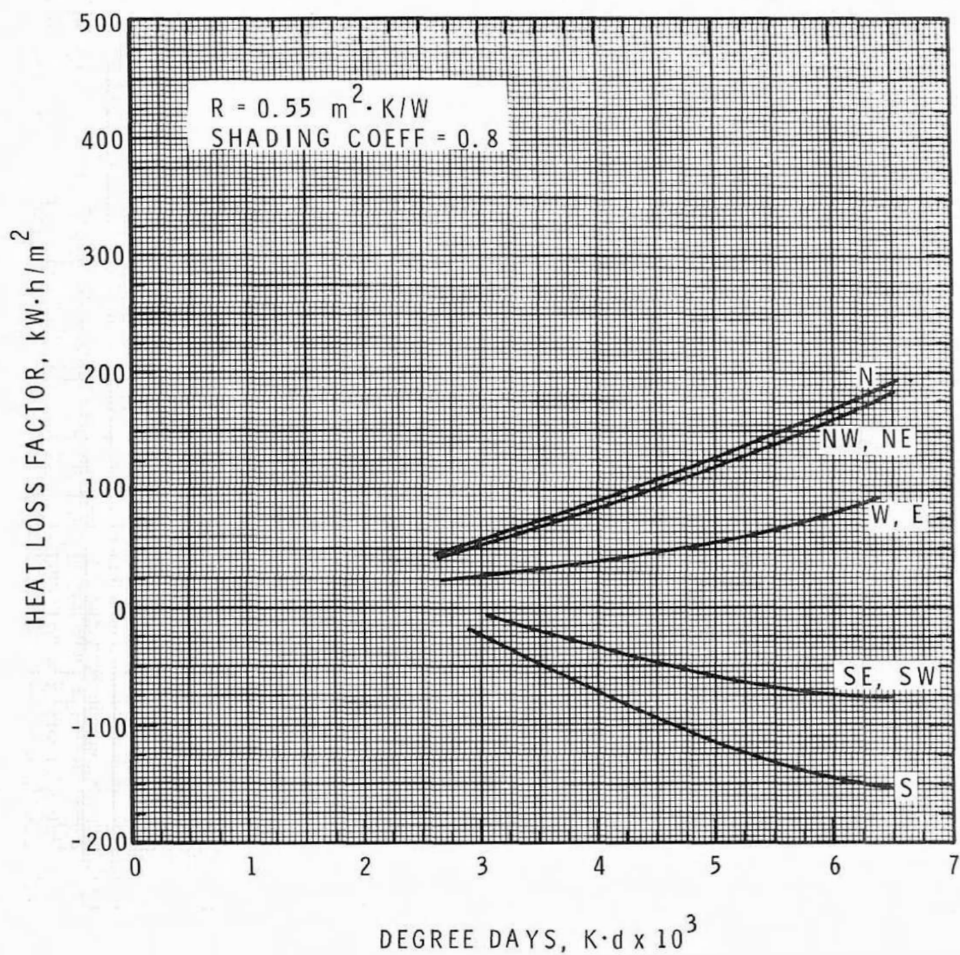
FIGURE 3 WINDOW HEAT LOSS FACTORS FOR TRIPLE GLAZING
