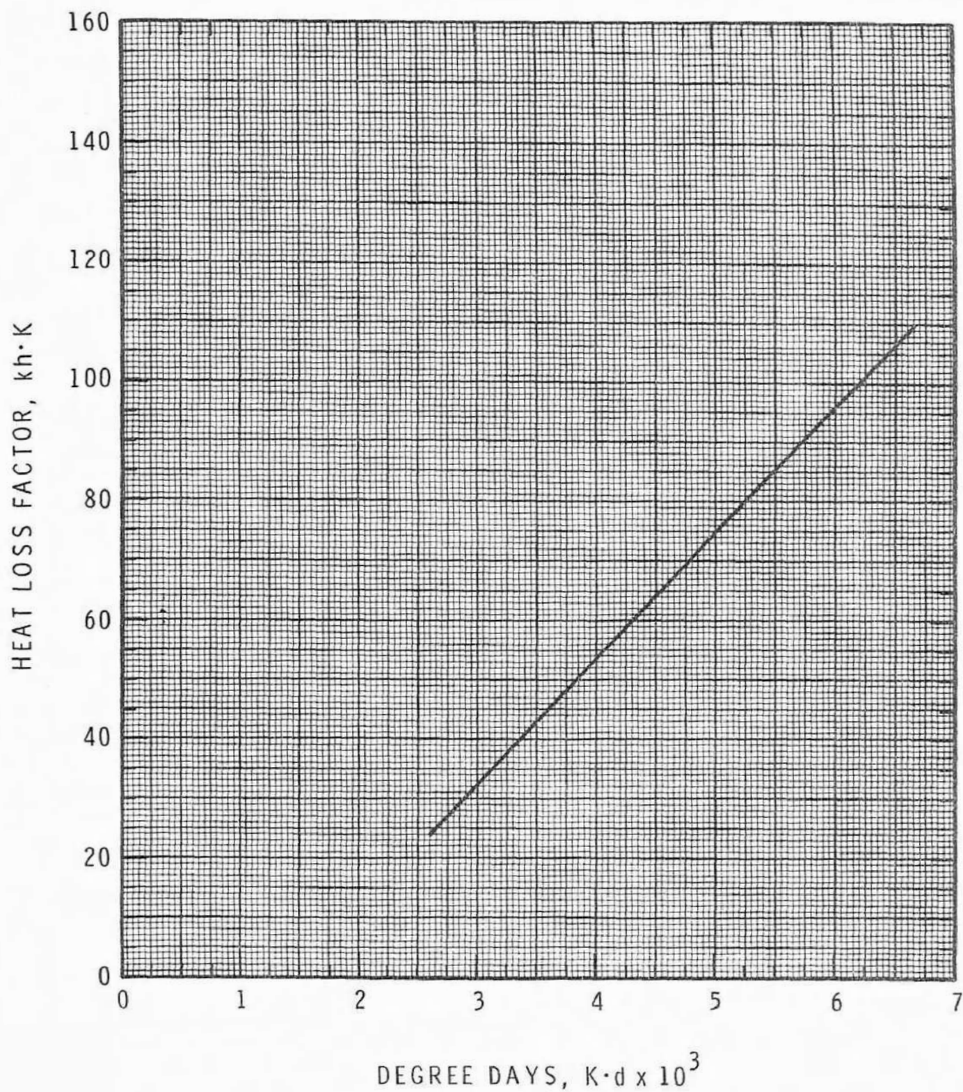
FIGURE 7 CEILING - ROOF HEAT LOSS FACTORS
