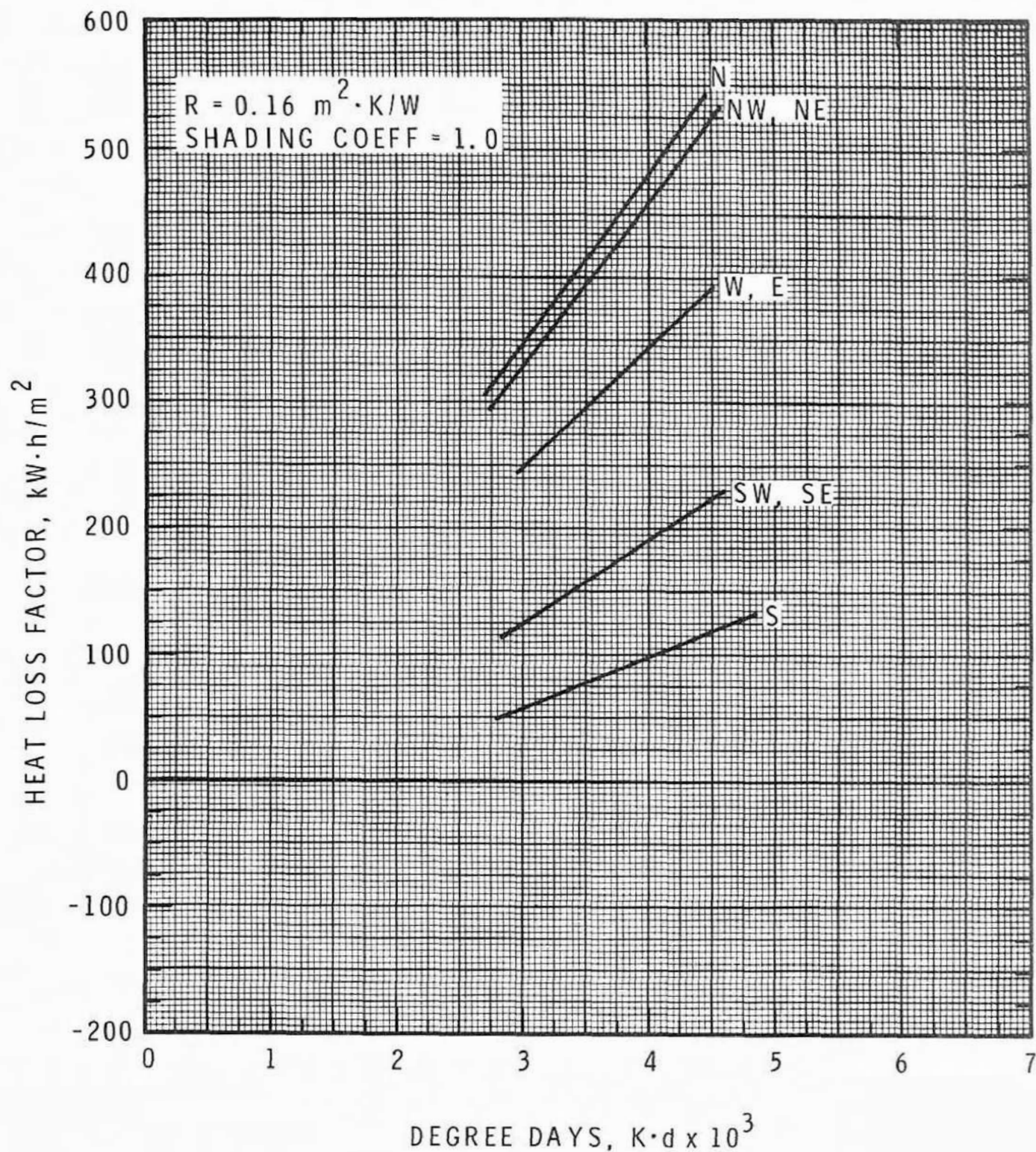
FIGURE 1 WINDOW HEAT LOSS FACTORS FOR SINGLE GLAZING
