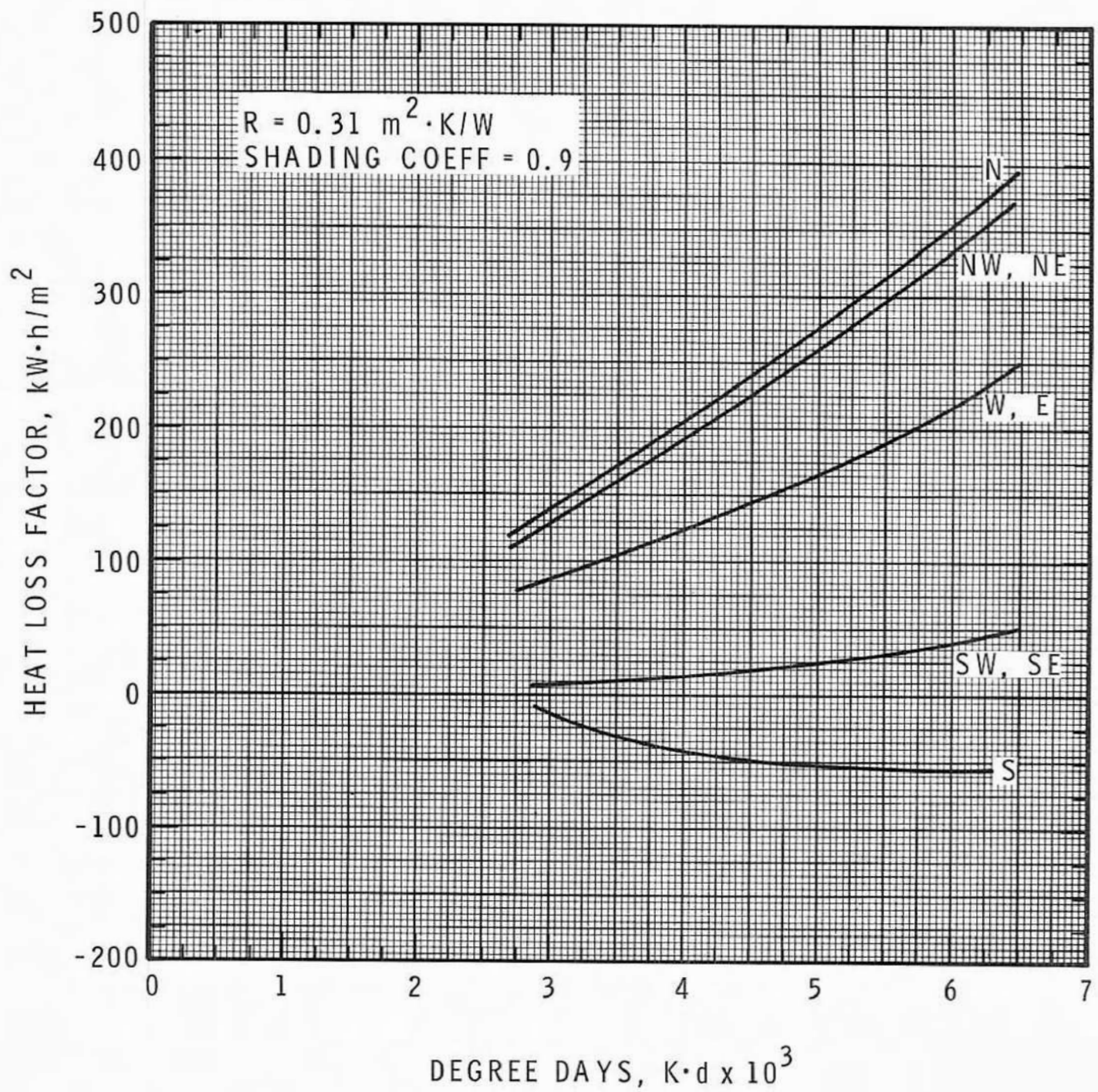
FIGURE 2 WINDOW HEAT LOSS FACTORS FOR DOUBLE GLAZING
