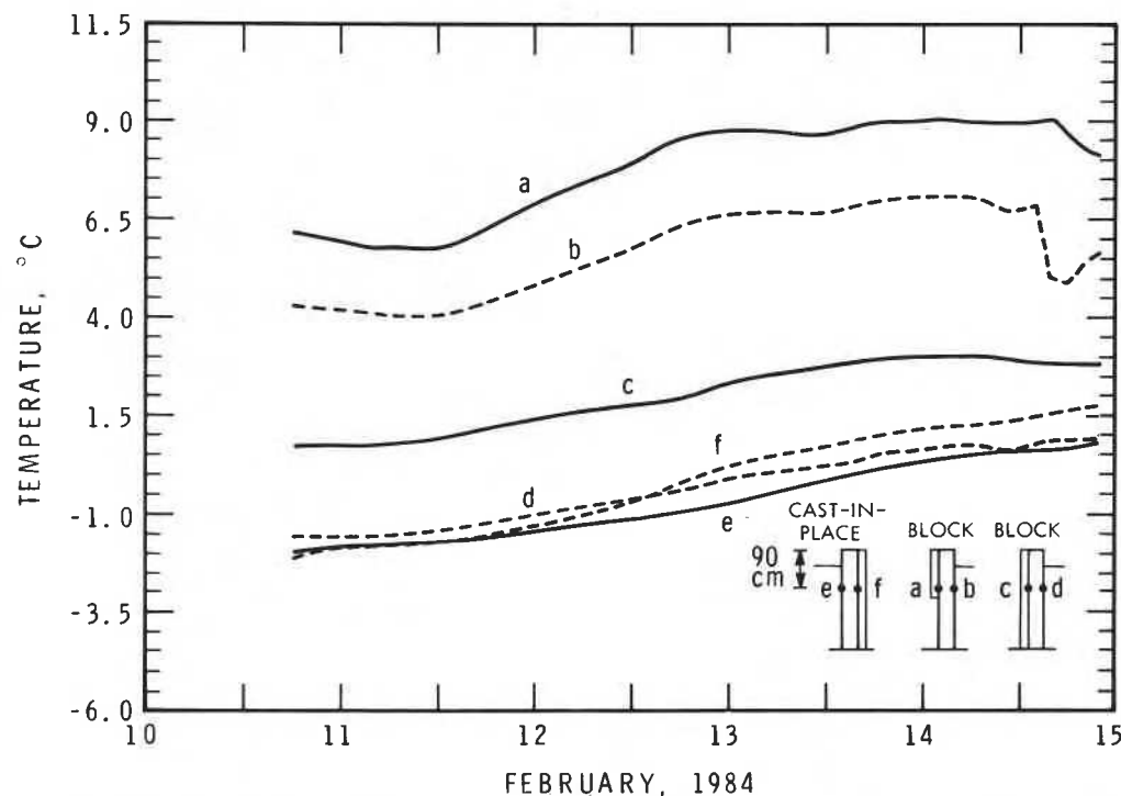
Figure 4 Temperatures of wall surfaces during warming trend.
