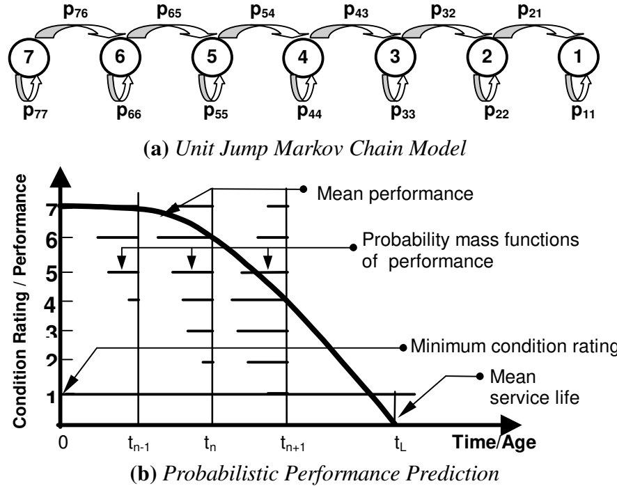
FIG. 2. Probabilistic Markovian Model for Performance Prediction
