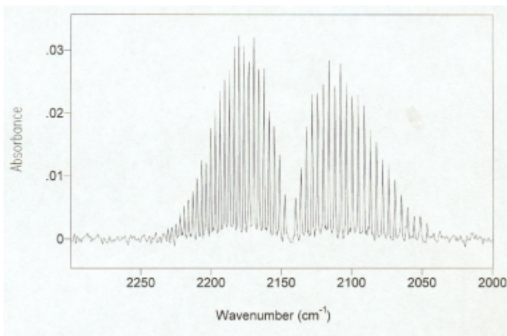
FIGURE 3. Carbon monoxide absorption band in FTIR calibration with 1091 ppm CO.
