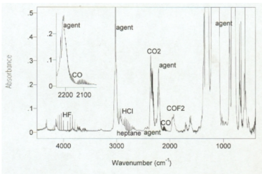
FIGURE 4. FTIR spectrum in an HCFC Blend A test.
