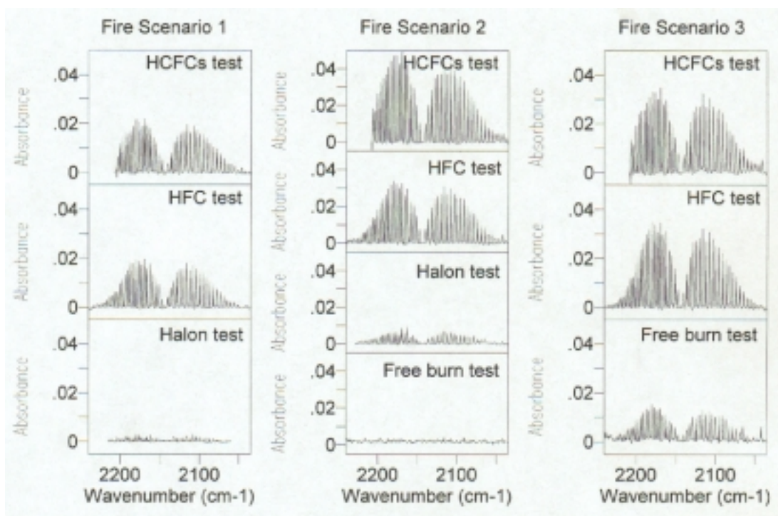
FIGURE 6. Average FTIR spectra of CO with baseline correction in fire tests.
