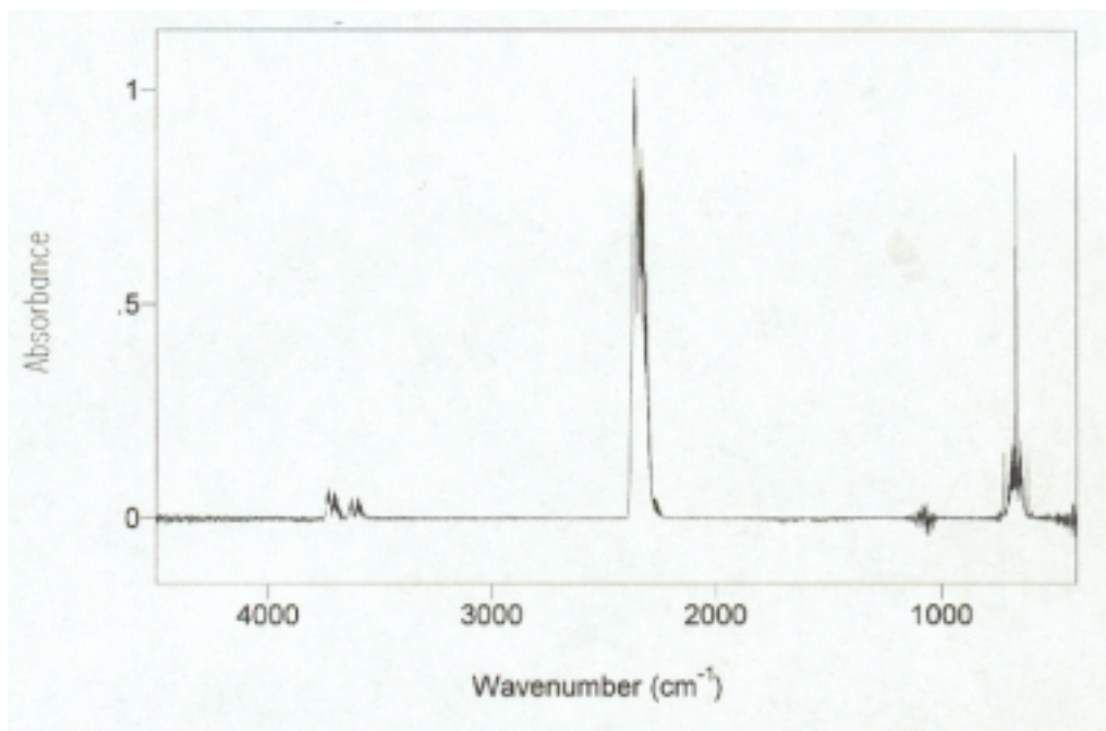
FIGURE 2. FTIR spectrum for the calibration of 2.23% carbon dioxide.
