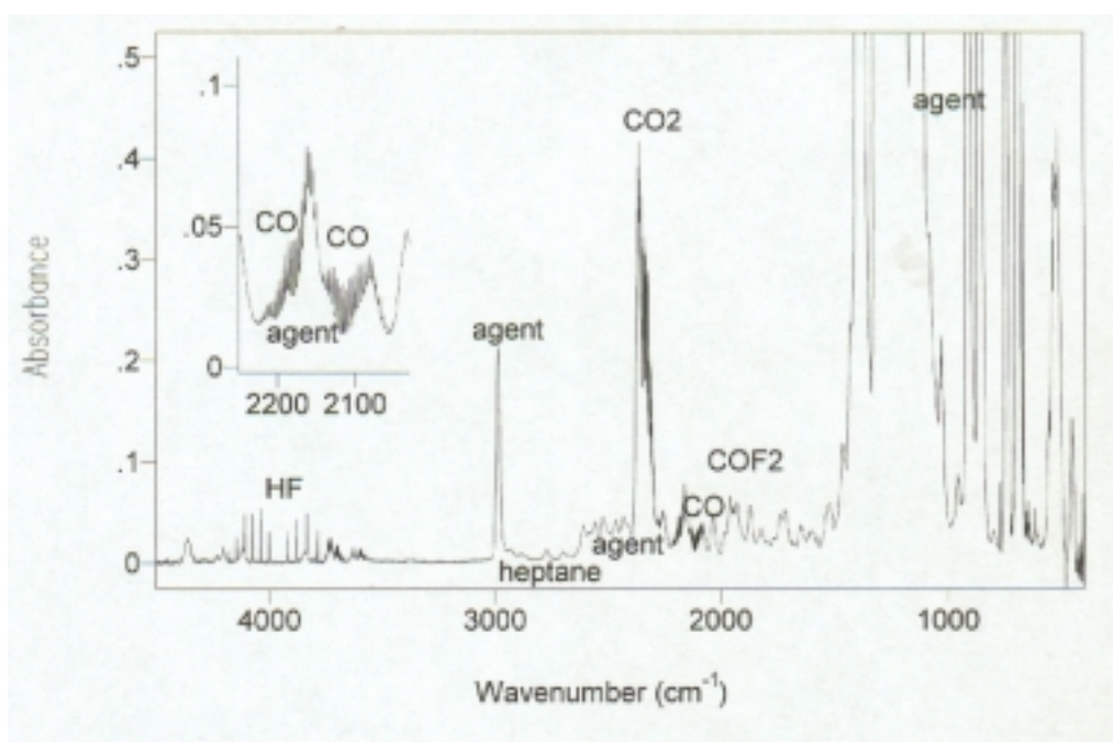
FIGURE 5. FTIR spectrum in an HFC-227ea test.
