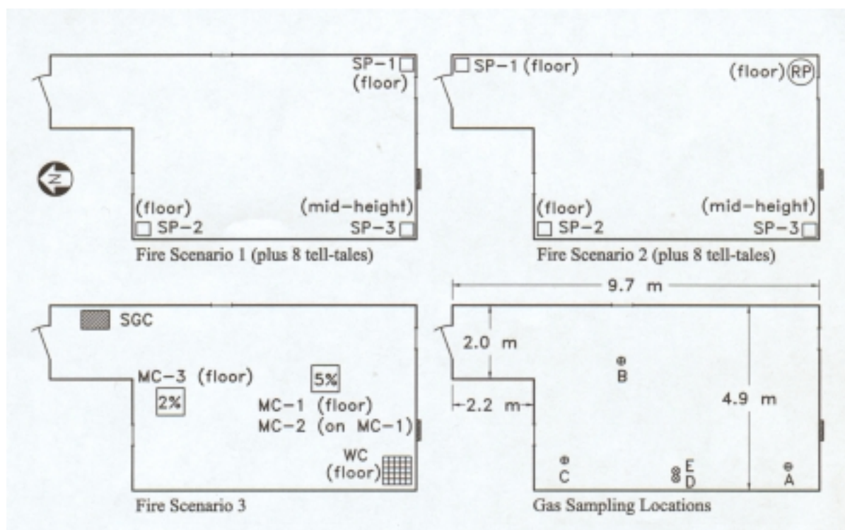
FIGURE 1. Plan view of test room, fire scenarios and locations, and gas sampling locations (⊕: A, B, C for FTIR; ⊗: D, E for nondispersive infrared analyzers).
