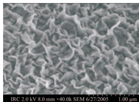
Fig. 1 SEM micrographs of synthetic C–S–H
