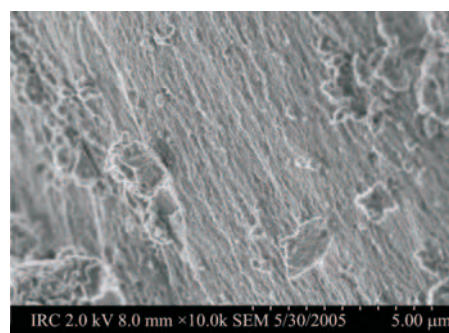
Fig. 2 SEM micrographs of intercalated C–S–HPN material (C–S–H–PAA (0.7–0.15))
