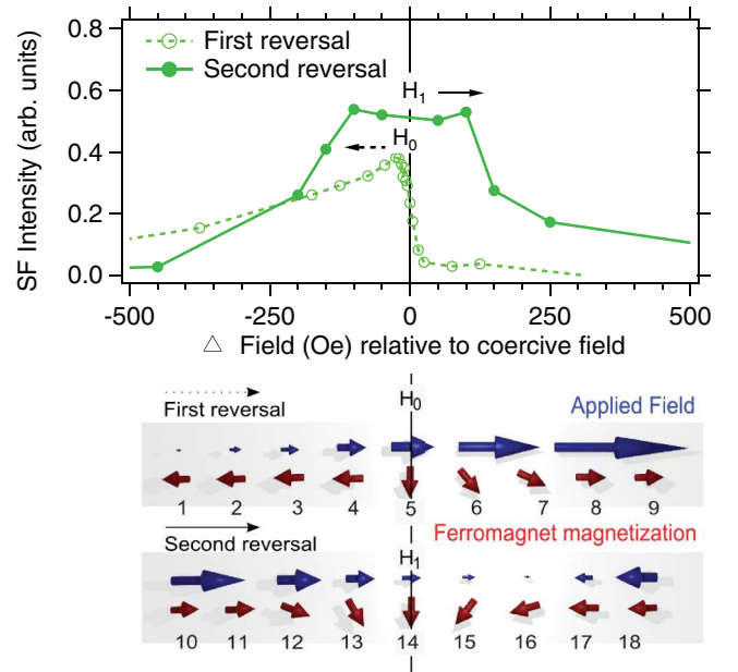
FIG. 15. (Color online) (Top) Integrated neutron spin-flip signal at fields near the coercive fields of first and second reversal points of the untrained loop, H_0 and H_1 . The larger neutron spin-flip intensity for the second reversal indicates a higher degree of coherence in the rotation with less loss of magnetization to domains parallel to the field. (Bottom) Simplified diagram of the sequence leading to the ferromagnetic spin-flop state at the first and second coercive fields H_0 and H_1 .
