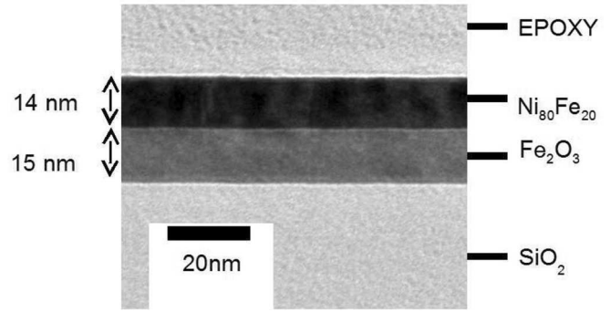
FIG. 1. Cross-sectional TEM image of Ni 80 Fe 20 / \alpha -Fe 2 O 3 film showing a uniform film with low interface roughness.
