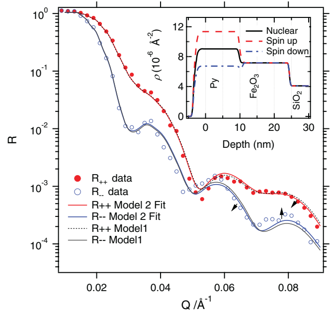
FIG. 8. (Color online) Room-temperature polarized neutron reflectometry patterns with fits according to model 1 and model 2 with parameters x = 1.0 nm, M = 0.75 \mu_B per Fe atom, as discussed in the text. Error bars lie within symbols. The arrows indicate the trend for how the two models differ.
