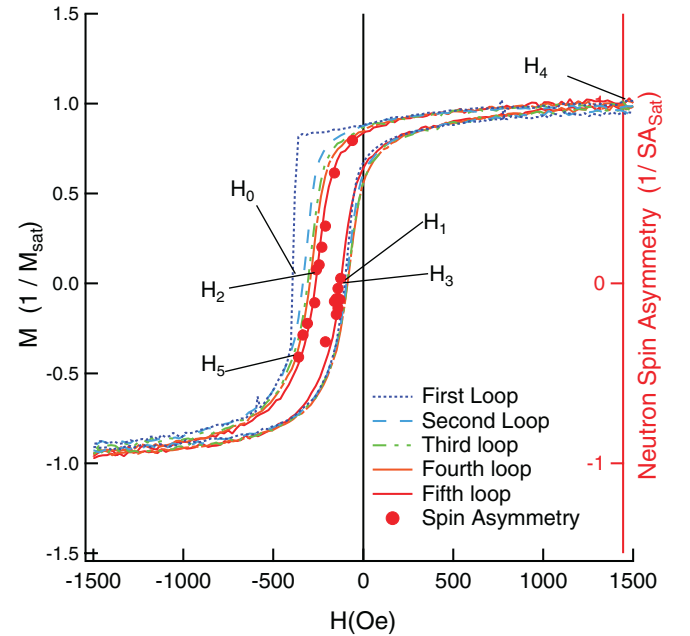
FIG. 13. (Color online) Magnetic training of permalloy/hematite interface at 5 K after field cooling from 300 K in +20 kOe. The neutron spin asymmetry (SA) at q = 0.028 \text{ \AA}^{-1} has been plotted over the trained magnetometry loop at 5 K. Both the spin asymmetry and magnetization have been normalized by the value measured at saturation.
