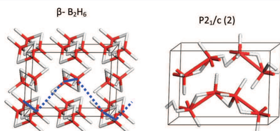
Figure 7. Structural interconversion between (left) the \beta diborane structure and (right) the P2_1/c (2) structure. Dashed lines highlight the traces in the molecular structures of the bonds that would complete the chain.
