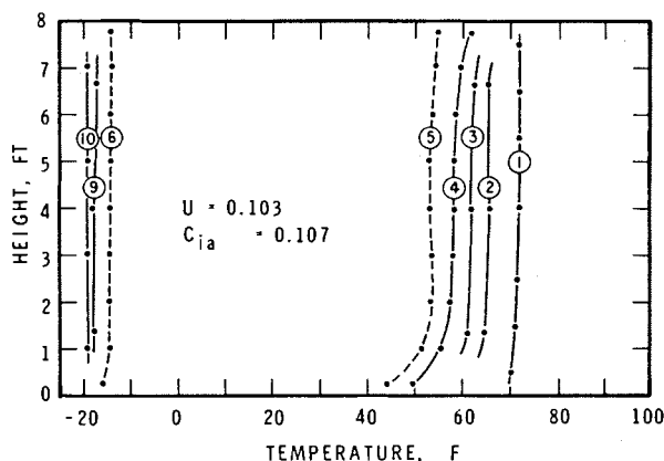
Fig. 8 Vertical temperature profiles, panel 2A1
