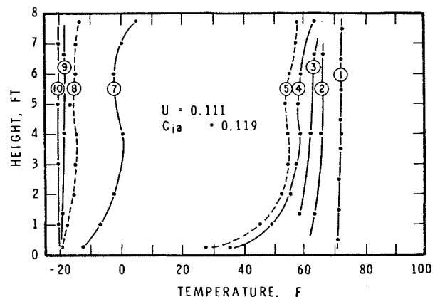
Fig. 9 Vertical temperature profiles, panel 2A4
