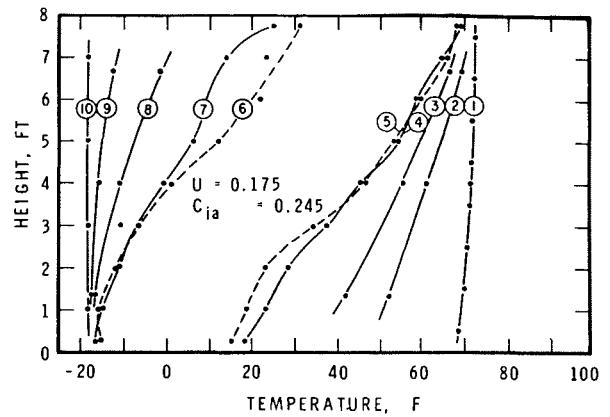
Fig. 7 Vertical temperature profiles, panel 1B2
