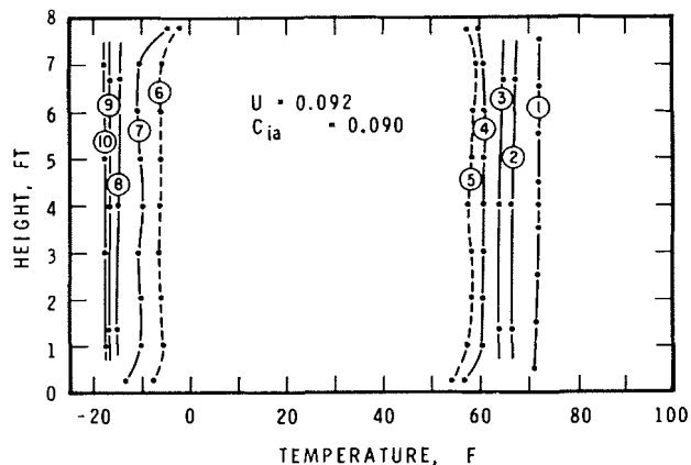
Fig. 4 Vertical temperature profiles, panel 1A1
