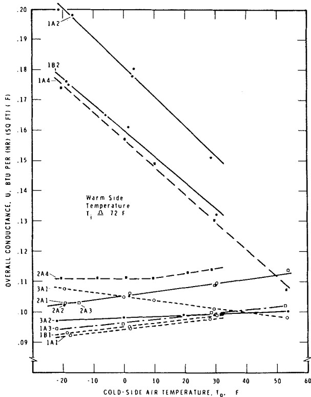
Fig. 10 Overall thermal conductance of panels
