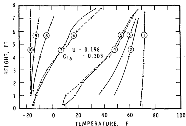
Fig. 5 Vertical temperature profiles, panel 1A2
