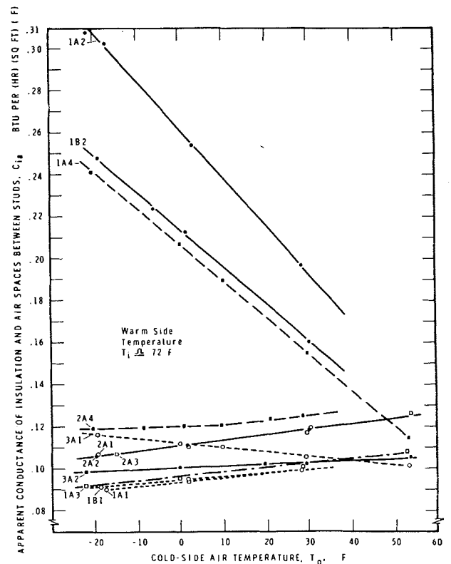
Fig. 11 Thermal conductance of insulation plus air spaces between studs
