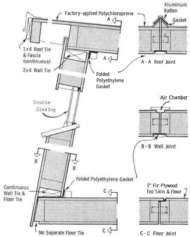
Fig. 2. Construction details, Angirraq hut.
