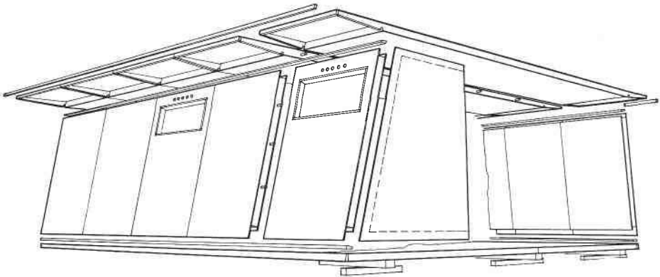
Fig. 1. Structural assembly of Angirraq hut.
