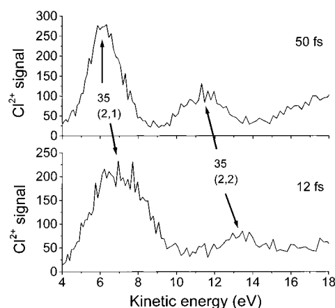
Figure 5. Kinetic energy spectrum of fragments created during the Coulomb explosion of \text{Cl}_2^+ and \text{Cl}_2^{2+} , for 50 fs (a) and 12 fs (b) pulses. For shorter pulses (i) positions of the peaks shift toward the Coulomb energy of explosion from the equilibrium position of the neutral, and (ii) peaks are significantly broader.
