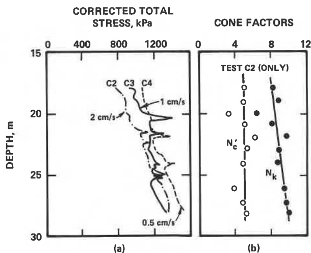
Figure 5. Corrected cone tip resistance profiles and cone factors.
