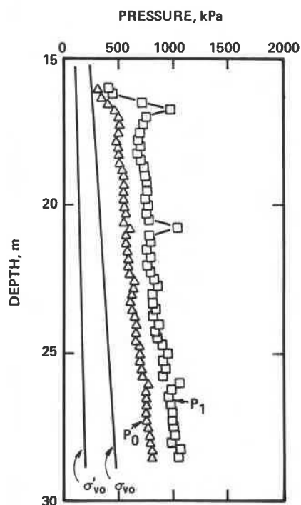
Figure 8. Dilatometer test results for DMT-6.
