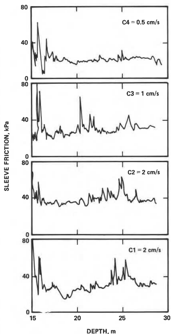
Figure 6. Measured sleeve friction for various cone penetration rates.
