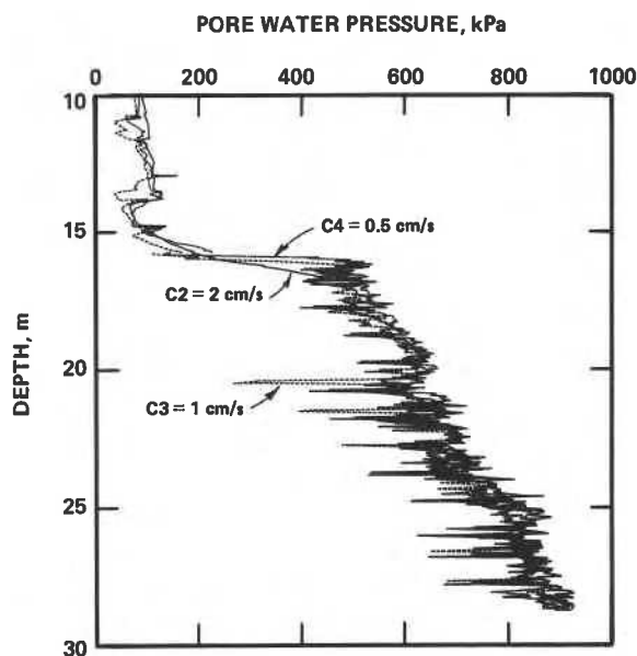
Figure 7. Excess pore water pressure profiles obtained at three different rates of penetration.
