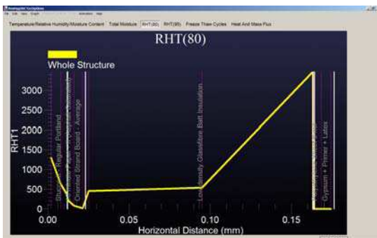
Figure 11. Output from 1-D hygIRC showing the final distribution of the accumulated total RHT (80) index through the entire wall section at the end of the simulation (a snapshot).
