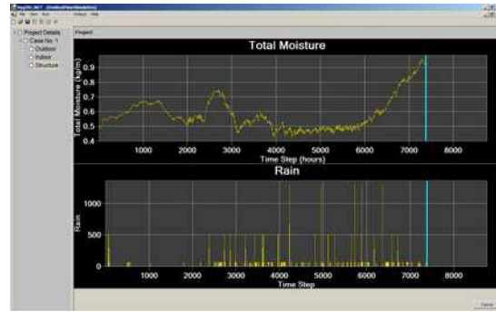
Figure 8. The screen shot shows the runtime operation of 1-D hygIRC. The real time history of the total moisture content for all the wall layers is shown here along with the real time history of rain events derived from the weather file.
