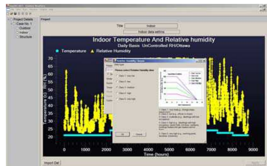
Figure 7. 1-D hygIRC also allows the relative humidity to be uncontrolled. Two models are provided: a statistical model and a model based on moisture generation rates. In this case a statistical model is assumed. The model assumes that the interior vapour pressure is equal to the exterior vapour pressure plus an amount determined by the occupancy and proportional to the mean monthly exterior temperature.
