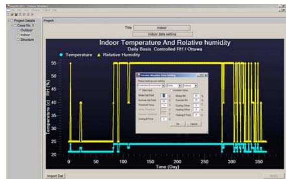
Figure 6. The interior condition models allow the user to set the interior temperature regimes using either a seasonal heating or daily balance point models. In this case the relative humidity is also controlled using set points.
