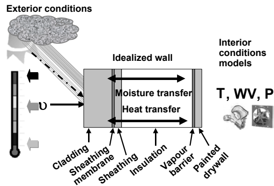
Figure 2. 1-D hygIRC is a one-dimensional simulation tool that models heat, air and moisture transfer through the various layers of 'virtual' building envelope components bounded on one side by the external environment and on the other by the indoor environment – 6 layers are shown
