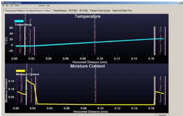
Figure 9. Output from 1-D hygIRC showing the final temperature and moisture content distribution through the entire wall section at the end of the simulation (a snapshot).
