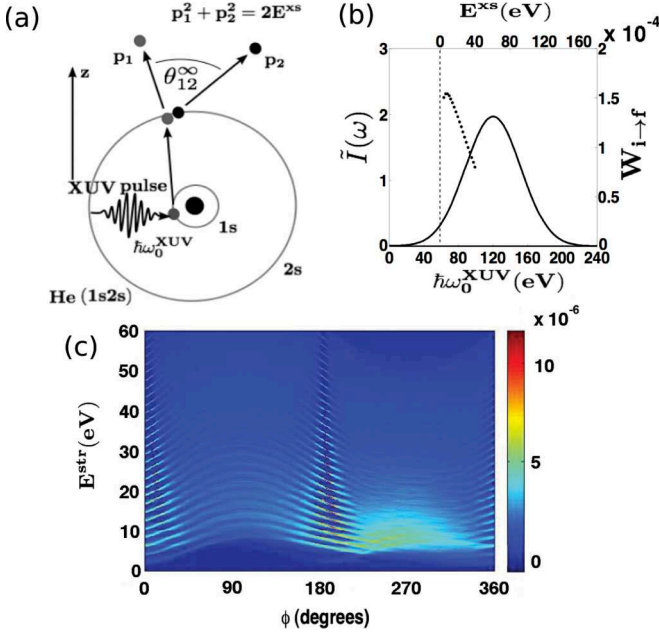
FIG. 1. (Color online) (a) Sketch of the intra-atomic knock-out mechanism to be studied with the two-electron streak camera. The streaking field causes a decrease in \theta_{12}^\infty when the photoelectron is launched along the +\hat{z} direction, since adding \Delta p_{\text{IR}} to each of the electron momenta results in \theta_{12} < \theta_{12}^\infty . (b) Spectral intensity of the XUV pulse scaled by (F_0^{\text{XUV}})^2 . Dotted curve: W_{i \rightarrow f} in the presence of the XUV and IR field averaged over all \phi 's. (c) Observable E^{\text{str}} total electron energy as a function of \phi considering excess energies from 4 to 60 eV in steps of 2 eV and double-ionization events corresponding to launching of the photoelectron ( 1s ) in the \pm\hat{z} direction for \phi ranging from 0^\circ to 180^\circ . To illustrate the difference between launching of the photoelectron in the +\hat{z} versus the -\hat{z} direction we plot the E^{\text{str}} corresponding to +\hat{z} for \phi ranging from 0^\circ to 180^\circ and the E^{\text{str}} corresponding to -\hat{z} for \phi ranging from 180^\circ to 360^\circ .
