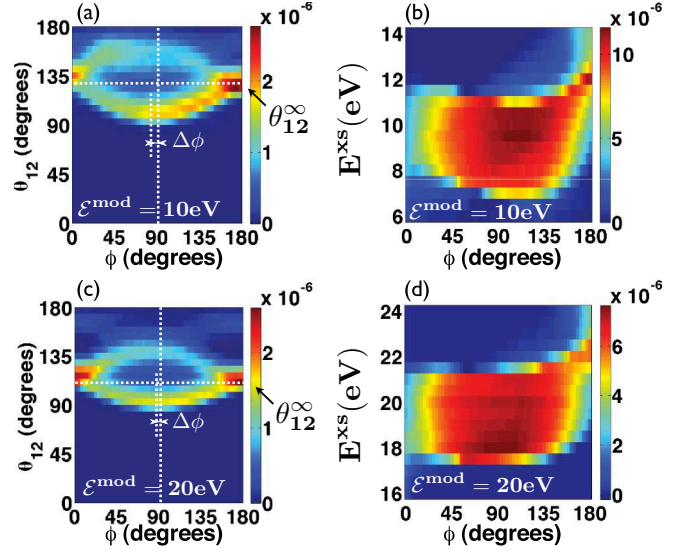
FIG. 4. (Color online) \theta_{12} as a function of \phi for “modified” energies around 10 eV (a) and 20 eV (c) in the presence of the XUV and IR field. \Delta\phi is the shift of the maximum of the vector potential of the IR field, corresponding to a maximum of the split of \theta_{12} as a function of \phi . (b) Excess energies as a function of \phi that contribute to the “modified” energy around 10 eV enclosed by the white dashed lines in Fig. 3(c) and similarly (not shown) for the “modified” energy centered around 20 eV. Figure 4 is plotted for symmetric E^{\text{mod}} energy sharing.
