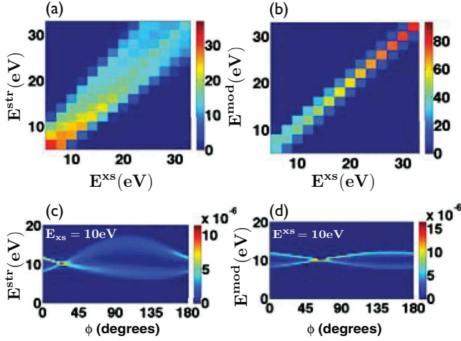
FIG. 2. (Color online) Correlation map of the excess energy E^{xs} (a) with the observable electron energy E^{str} and (b) with the “modified” electron energy E^{mod} . The color scale in panels (a) and (b) is such that the sum of E^{xs} contributing to a certain E^{str} is normalized to 100. (c) Streaked electron energy and (d) “modified” electron energy as a function of \phi for E^{xs} = 10 eV excess energy. Panels (a) and (c) are plotted for symmetric E^{str} energy sharing while panels (b) and (d) are plotted for symmetric E^{mod} energy sharing.
