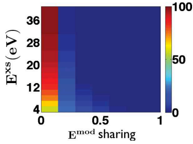
FIG. 6. (Color online) Correlation map of the excess energy with the “modified” energy sharing for the doubly ionizing events with equal energy sharing in the absence of the IR field. The color scale is such that the sum of E^{\text{mod}} energy sharings contributing to the equal energy sharing double-ionization events for a certain E^{\text{xs}} is normalized to 100.
