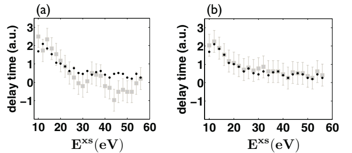
FIG. 5. \square indicates the collision times for “modified” electron energies \mathcal{E}^{\text{mod}} from 10 to 56 eV; \bullet indicates the collision times for pure excess energies E^{\text{xs}} ranging from 10 to 56 eV. Collision time was retrieved by (a) method 1 and (b) method 2. The error bars show the uncertainty in the delay times of 0.6 a.u. since we change \phi every 1^\circ .
