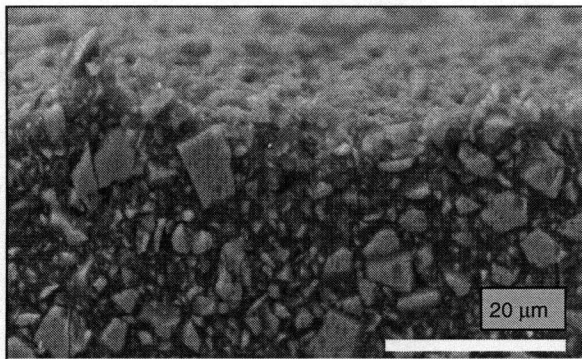
Figure 6b: SEM micrograph of a perpendicular cut of the eroded surface; Epoxy without nanoclay and side view with an angle.
