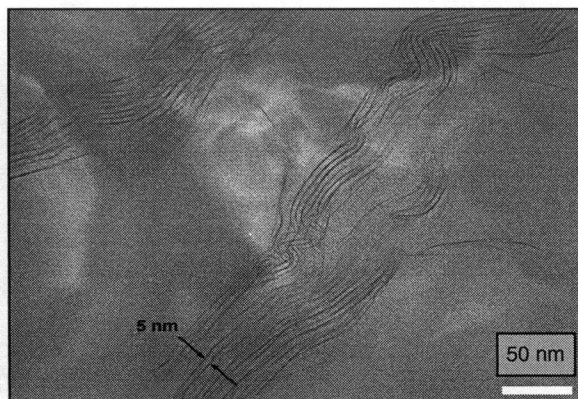
Figure 7c: TEM micrograph of the epoxy containing nanoclay showing the well dispersed platelets of aluminosilicates.
