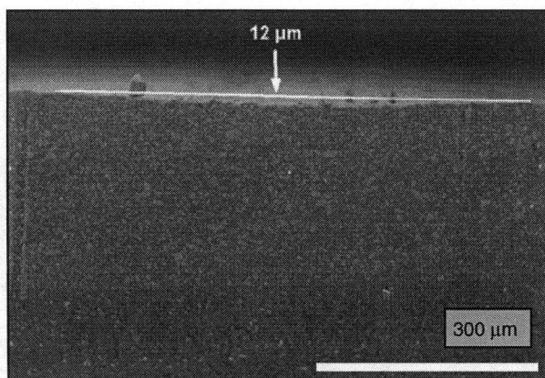
Figure 6a: SEM side view of a perpendicular plane to the eroded surface of the epoxy without nanoclay.
