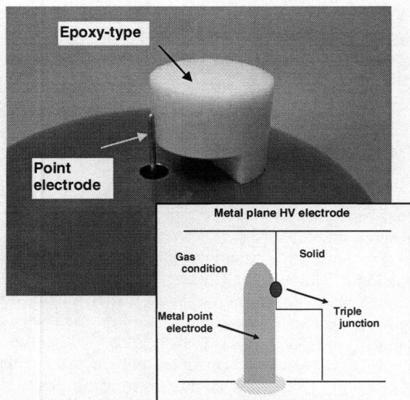
Figure 1: View of the experimental electrode arrangement and schematical definition of the triple junction.
