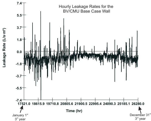
Figure 6. Air leakage rates analysis. Positive-negative leakage rates means air infiltration-exfiltration
