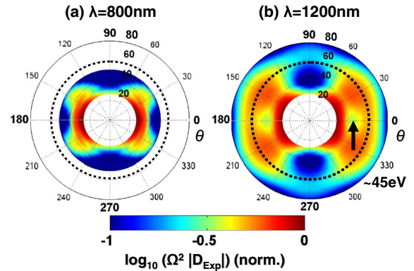
FIG. 2 (color online). Experimental molecular frame transition moments in aligned \text{N}_2 , derived from the results in Fig. 1. We display the extracted amplitude \Omega^2 |\vec{D}_{\text{Exp}}(\Omega, \theta)| by deconvolving the molecular alignment distribution using Eq. (1). While the laboratory frame signal peaks at \alpha = 0^\circ (see Fig. 1) across the spectrum, in the molecular frame the amplitude instead peaks at a significant angle ( \theta \sim 35^\circ ) between the molecular axis and the laser polarization above 40 eV at 800 nm and at 45 \pm 5 \text{ eV} at 1200 nm.
