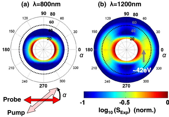
FIG. 1 (color online). Experimentally recorded high-harmonic signal from aligned \text{N}_2 as a function of alignment angle \alpha for two probe-pulse central wavelengths (800 or 1200 nm) at I_{\text{probe}} = 1.5 \times 10^{14} \text{ W/cm}^2 . The radius of the polar plots corresponds to photon energies in the range of 0–80 eV, while the angle corresponds to the angle \alpha between the probe polarization and the molecular alignment. The black dotted line marks 60 eV. The color scale is logarithmic.
