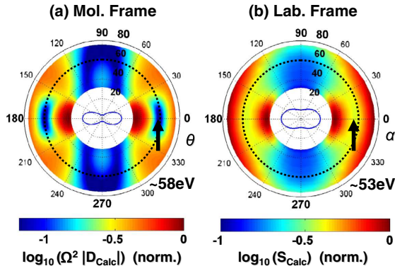
FIG. 3 (color online). Theory: (a) Molecular frame high harmonic amplitude \Omega^2|\vec{D}_{\text{calc}}(\Omega, \theta)| using calculated differential photoionization dipole matrix elements and analytical angular ionization probabilities. (b) Expected laboratory frame XUV signal S_{\text{calc}}(\Omega, \theta) using Eqs. (1) and (2) to convolve the calculated molecular frame values from (a) with the experimental alignment distribution. The solid line in the middle is the normalized ionization rate in the respective frames calculated using molecular Ammosov-Delone-Krainov rates. The alignment averaging shifts the spectral minimum at \theta = 0^\circ towards lower photon energy and reduces its depth, as seen experimentally.
