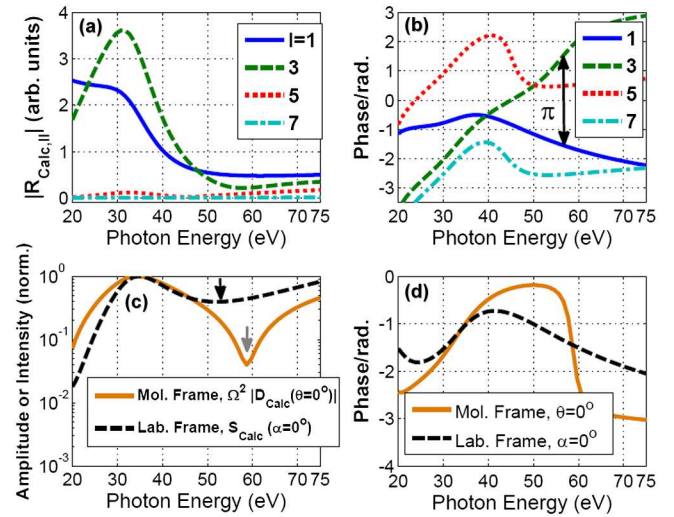
FIG. 4 (color online). Decomposing the calculated photorecombination dipole R_{\text{calc},\parallel}(\theta = 0^\circ) into contributions from the different partial spherical waves ( l ) describing the continuum \Sigma_u state in aligned ( \theta = 0^\circ ) \text{N}_2 : (a) their relative amplitudes and (b) phases. A \pi phase difference between the dominant l = 1 and 3 ( p and f waves) components explains the strong spectral minimum at \sim 58 eV. This molecular electronic structural minimum is analogous to the Cooper minimum probed in argon [27] by high harmonic generation. (c–d) The calculated amplitude (c) and phase (d) in the molecular frame (solid line) and in the laboratory frame (dashed line).
