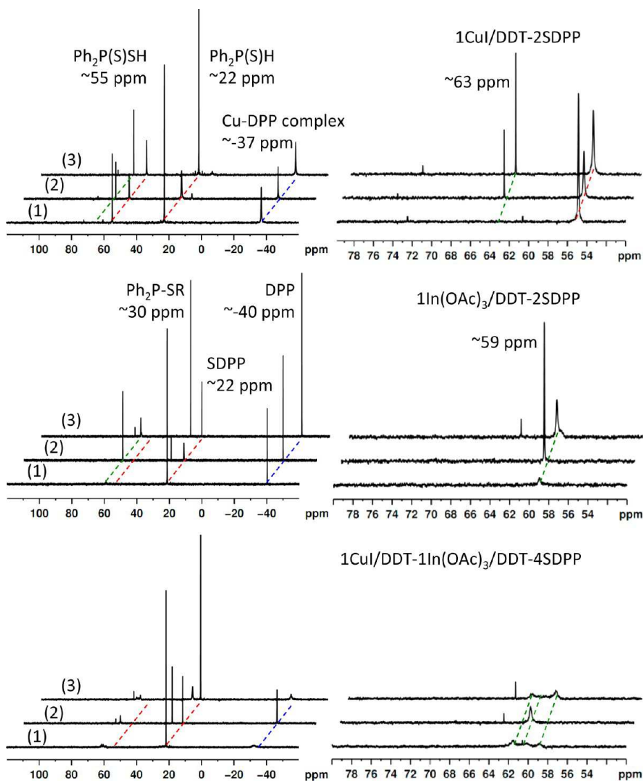
Figure 2. In situ ^{31}\text{P} NMR with ^1\text{H} decoupling of three reactions of 1\text{CuI/DDT-2SDPP} with [\text{Cu}] \sim 74 \text{ mmol/kg} (top), 1\text{In(OAc)}_3/\text{DDT-2SDPP} with [\text{In}] \sim 21 \text{ mmol/kg} (middle), and 1\text{CuI/DDT-1In(OAc)}_3/\text{DDT-4SDPP} with [\text{Cu} + \text{In}] \sim 38 \text{ mmol/kg} (bottom). The spectra (left) were collected when the temperature was increased from 30^\circ\text{C} (1) to 100^\circ\text{C} (2) and back to 30^\circ\text{C} (3), as indicated. The regions of 50\text{--}80 \text{ ppm} in the right panel display probable Cu–S and In–S complexes formed.
