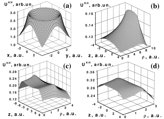
FIG. 2. Average potential U^{\text{KH}} : (a) binding in 2D ( a = 3 a.u.); (b) “weak” linear field b/a < \kappa_0 ( b = 2 a.u., a = 8 a.u.)—the repulsion is along the z axis; (c) “strong” linear field b/a > \kappa_0 ( b = 8 a.u., a = 2 a.u.)—the repulsion is in the radial direction; (d) for b/a = \kappa_0 ( b \approx 4.36 a.u., a = 2 a.u.) the potential is flat inside the cylinder.
