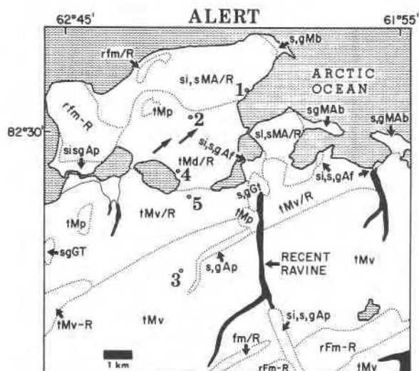
FIGURE 3. Map of surficial geology showing the general distribution of the sediments of glacial, glaciofluvial, marine, and bedrock origin. The temperature measurement sites are shown (numbers 1 to 5).
